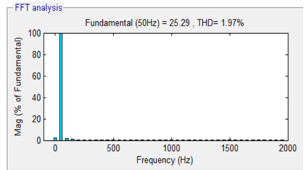
Fig 10: Total Harmonics distortion of source currents.
