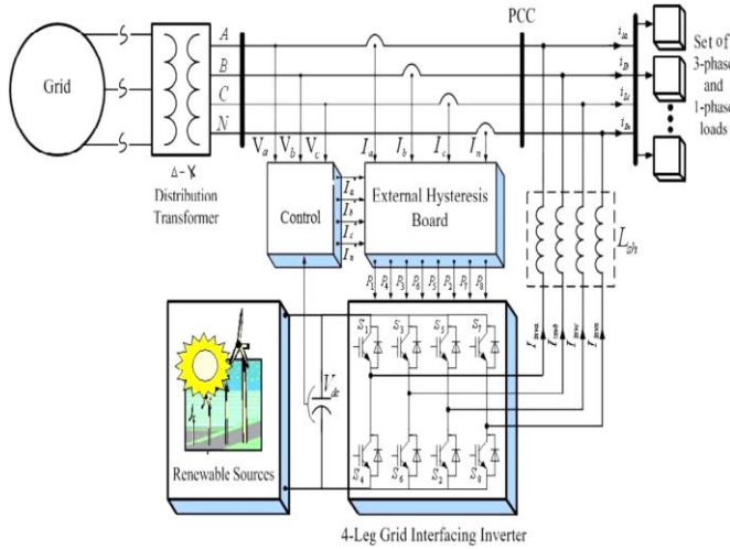
Fig.1. Block diagram of grid connected wind generation system at distribution level
