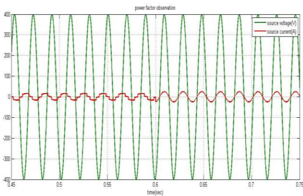
Fig 8: Power factor maintained unity when the STATCOM is acting from 0.6 sec.
