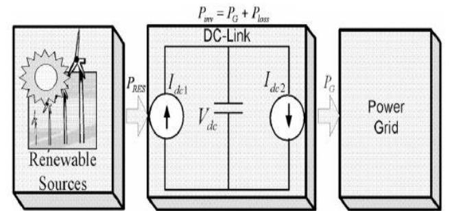
Fig.2. DC-Link Equivalent Diagram.
