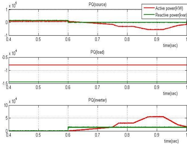
Fig 7: Simulated output wave forms of Source, load and Compensated active and re-active powers.
