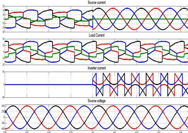
Fig 6: Three phase wave forms of source current, Load current, inverter currents and source voltage
