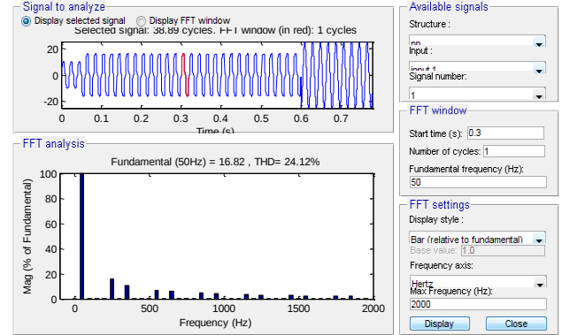
Fig.9: Total Harmonics distortion of source current
