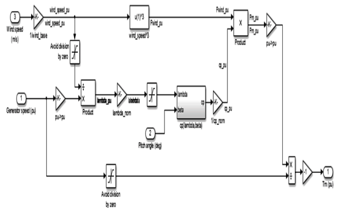
Fig.5: Simulink model of wind turbine
