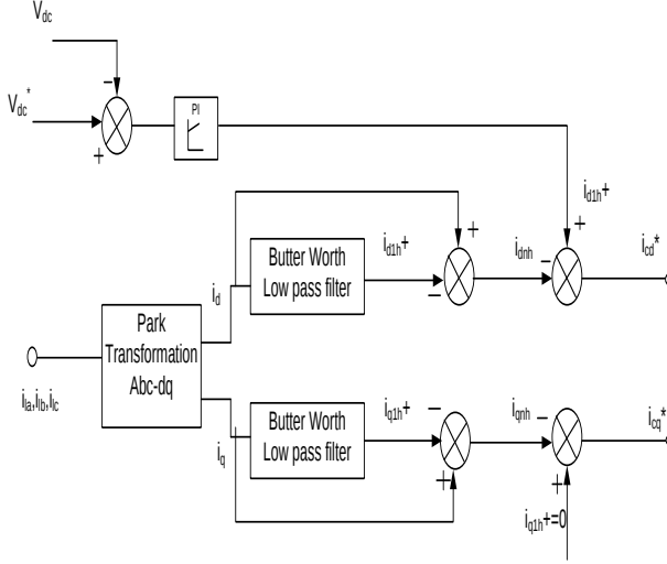
Fig.3. Transformation and injection of harmonic current
